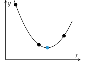
Figure 3.10. Quadratic fit search fits a quadratic function to three bracketing points (black dots) and uses the analytic minimum (blue dot) to determine the next set of bracketing points.
