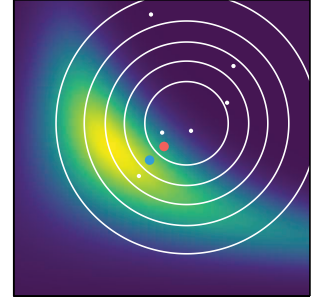
Figure 8.8. Shown is an initial proposal distribution (white contours), six samples (white dots), and the new updated means for both covariance matrix adaptation (blue dot) and the cross-entropy method (red dot) using three elite samples. Covariance matrix adaptation tends to update the mean more aggressively than the cross-entropy method (red dot), as it assigns higher weight to better sampled designs.
