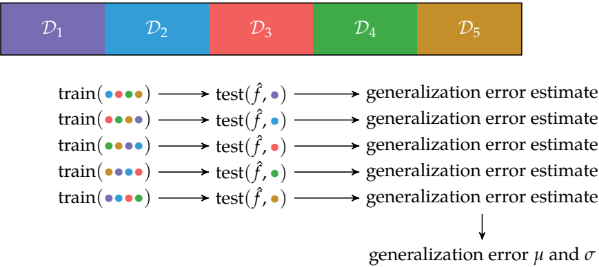
Figure 14.10. Cross-validation partitions the data into equally sized sets. Each set is the holdout set once. Here we show 5-fold cross-validation.
