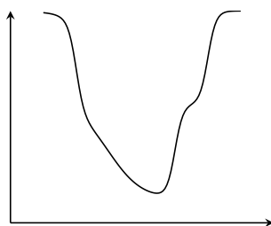
Unimodal but nonconvex
