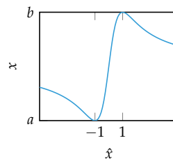
Figure 10.4. This transform ensures that x lies between a and b .
