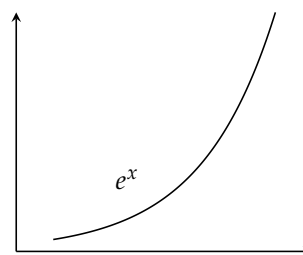
Convex but nonunimodal
