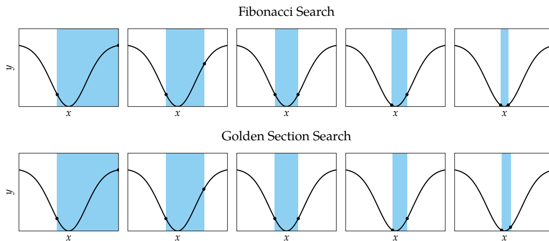
Figure 3.8. Fibonacci and golden section search on a unimodal function.
