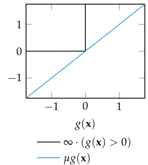
Figure 10.7. The linear function \mu g(\mathbf{x}) is a lower bound to the infinite step penalty so long as \mu \geq 0 .
