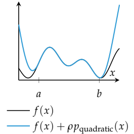
Figure 10.9. Using a quadratic penalty function for minimizing f subject to x \in [a, b] .
