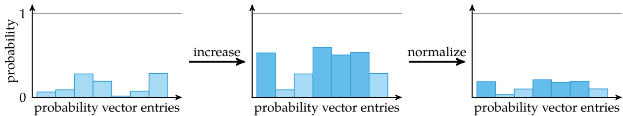
Figure 20.10. Mutating a probability vector in a probabilistic prototype tree with \beta = 0.5 . The mutated components were increased according to equation (20.5) and the resulting probability vector was renormalized. Notice how smaller probabilities receive greater increases.
