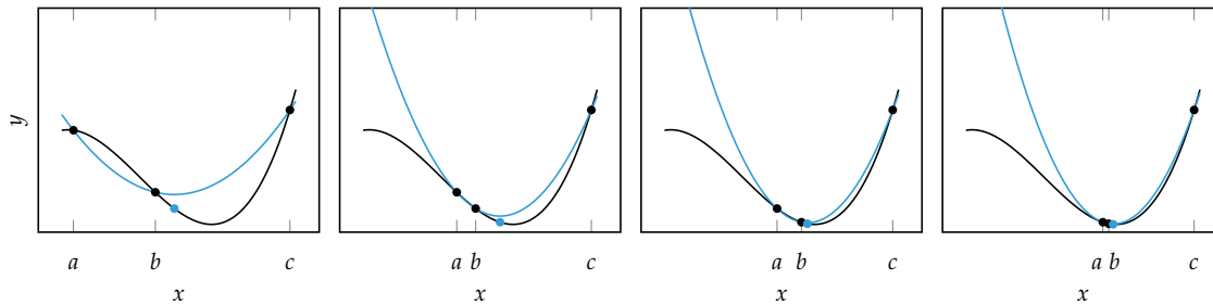
Figure 3.11. Four iterations of the quadratic fit method.
