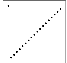
Figure 13.11. The Halton sequence with b = [19, 23] for which the first 18 samples are perfectly linearly correlated.
