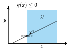
Figure 17.6. Optima with active constraints are often sensitive to uncertainty.
