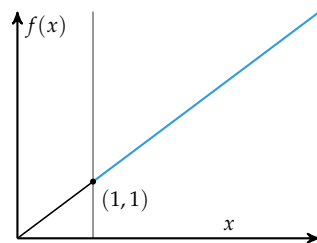
Figure 1.5. The problem in equation (1.6) has no solution because the constraint boundary is not feasible.
