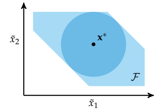
Figure 17.3. Information-gap decision theory applied to an objective function with additive noise f(\tilde{\mathbf{x}}) with \tilde{\mathbf{x}} = \mathbf{x} + \mathbf{z} and a circular uncertainty set
