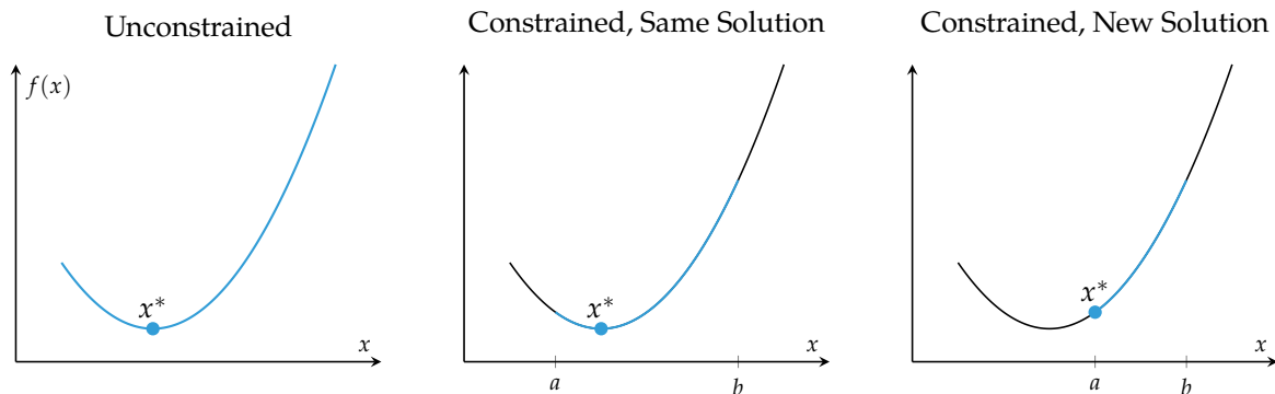
Figure 10.3. Constraints can change the solution to a problem, but do not have to.
