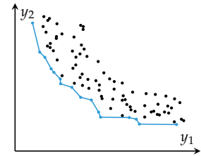
Figure 12.4. Generating Pareto frontiers with naively scattered points is straightforward but inefficient and approximate.
