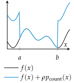
Figure 10.8. The original and count-penalized objective functions for minimizing f subject to x \in [a, b] .
