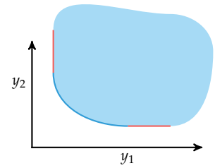
Figure 12.3. Weakly Pareto-optimal points, shown in red, cannot be improved simultaneously in all objectives.
