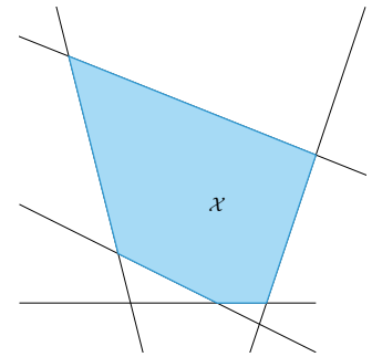
Figure 11.3. The intersection of linear constraints is a convex set.
