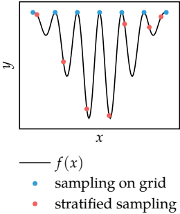
Figure 13.5. Using an evenly-spaced grid on a function with systematic regularities can miss important information.
