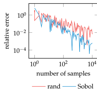
Figure 13.10. The error from estimating \int_0^1 \sin(10x) dx using Monte Carlo integration with random numbers from U(0, 1) and a Sobol sequence. The Sobol sequence, covered in section 13.7.3, converges faster.
