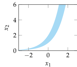
Figure D.1. The noise-free feasible region.
