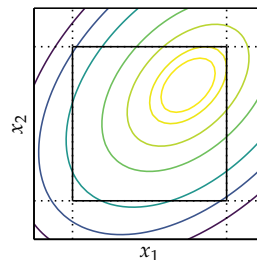
Figure 10.2. Bracketing constraints force the solution to lie within a hyperrectangle.
