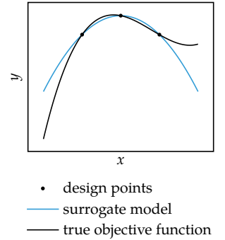
Figure 14.1. Surrogate models approximate the true objective function. The model is fitted to the evaluated design points but deviates farther away from them.
