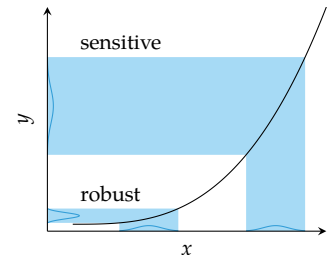
Figure 17.4. Probabilistic approaches produce probability distributions over the model output. Design points can be sensitive or robust to uncertainty. The blue regions show how the distribution over a normally distributed design is affected by the objective function.
