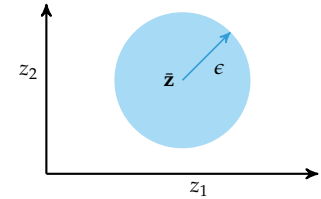
Figure 17.2. A parametrized uncertainty set \mathcal{Z}(\epsilon) in the form of a hypersphere.
