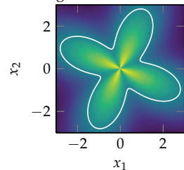
Figure 16.13. SafeOpt applied to the flower function (appendix B.4) with y_{\max} = 2 , a Gaussian process mean of \mu(\mathbf{x}) = 2.5 , variance \nu = 0.01 , \beta = 10 , a 51 \times 51 uniform grid over the search space, and an initial point \mathbf{x}^{(1)} = [-2.04, 0.96] . The color indicates the value of the upper bound, the cross indicates the safe point with the lowest upper bound, and the white contour line is the estimated safe region.
