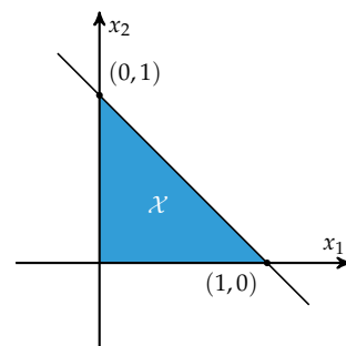
Figure 1.4. The feasible set \mathcal{X} associated with equation (1.5).
